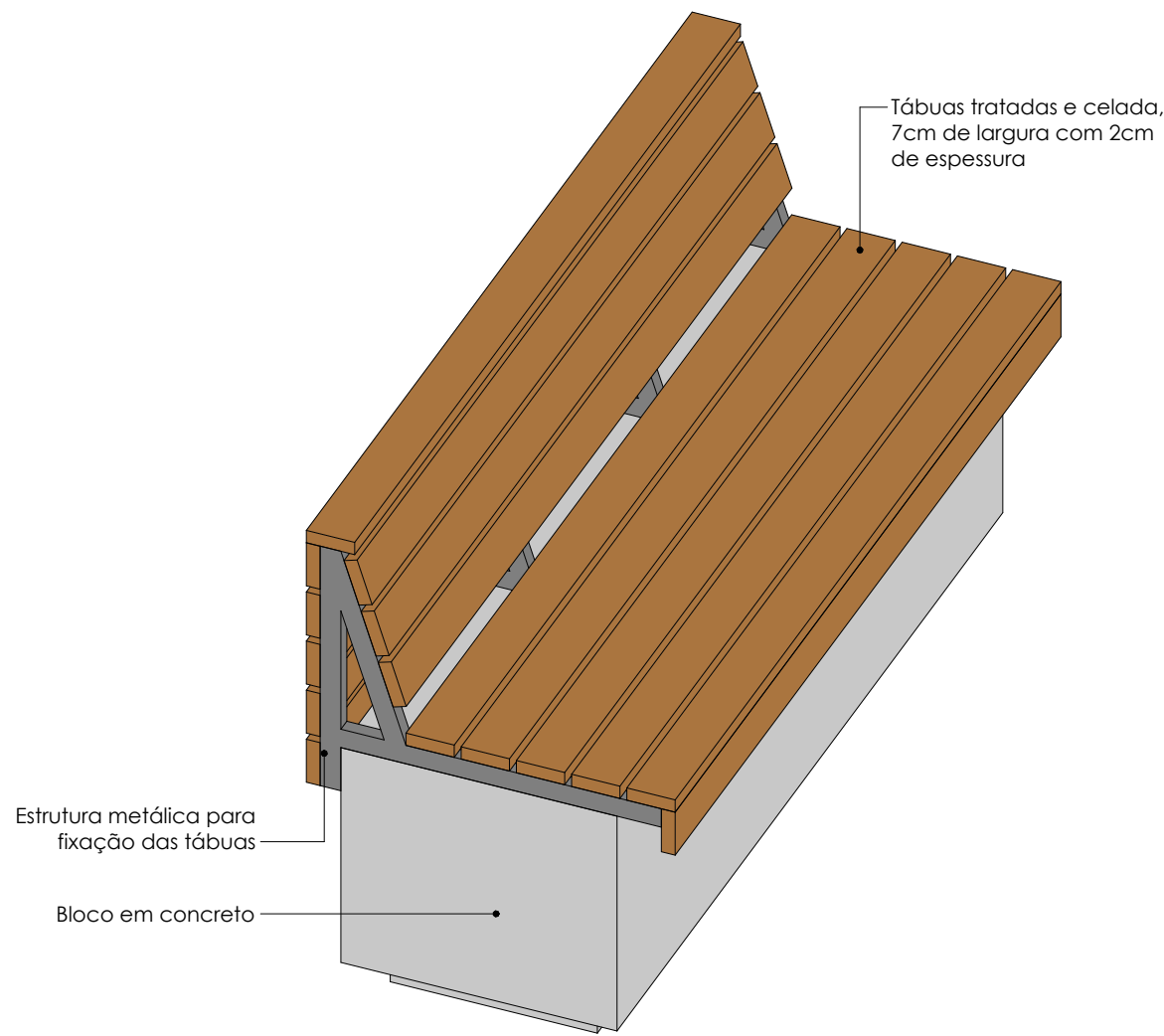
4 Ortogonal 3D
