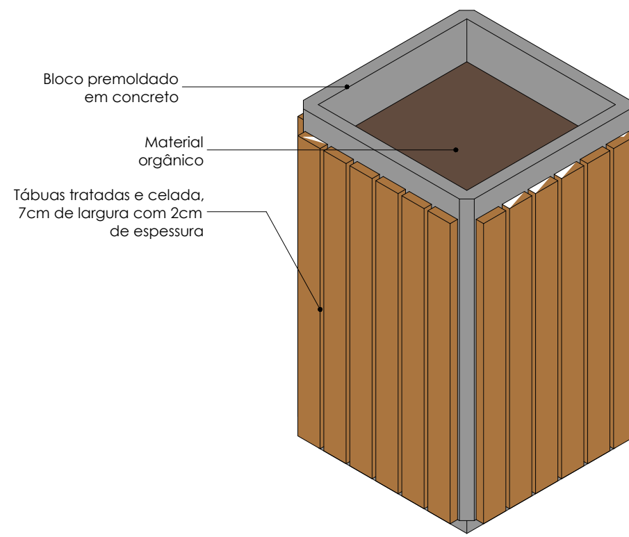
12 Ortogonal 3D
