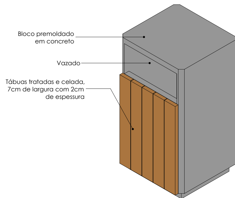
8 Ortogonal 3D
